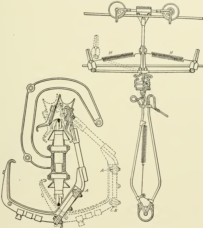
Fig. 13. Details of Trolley Suspension and Current Collector of the Koehler System Courtesy of Engineering News
